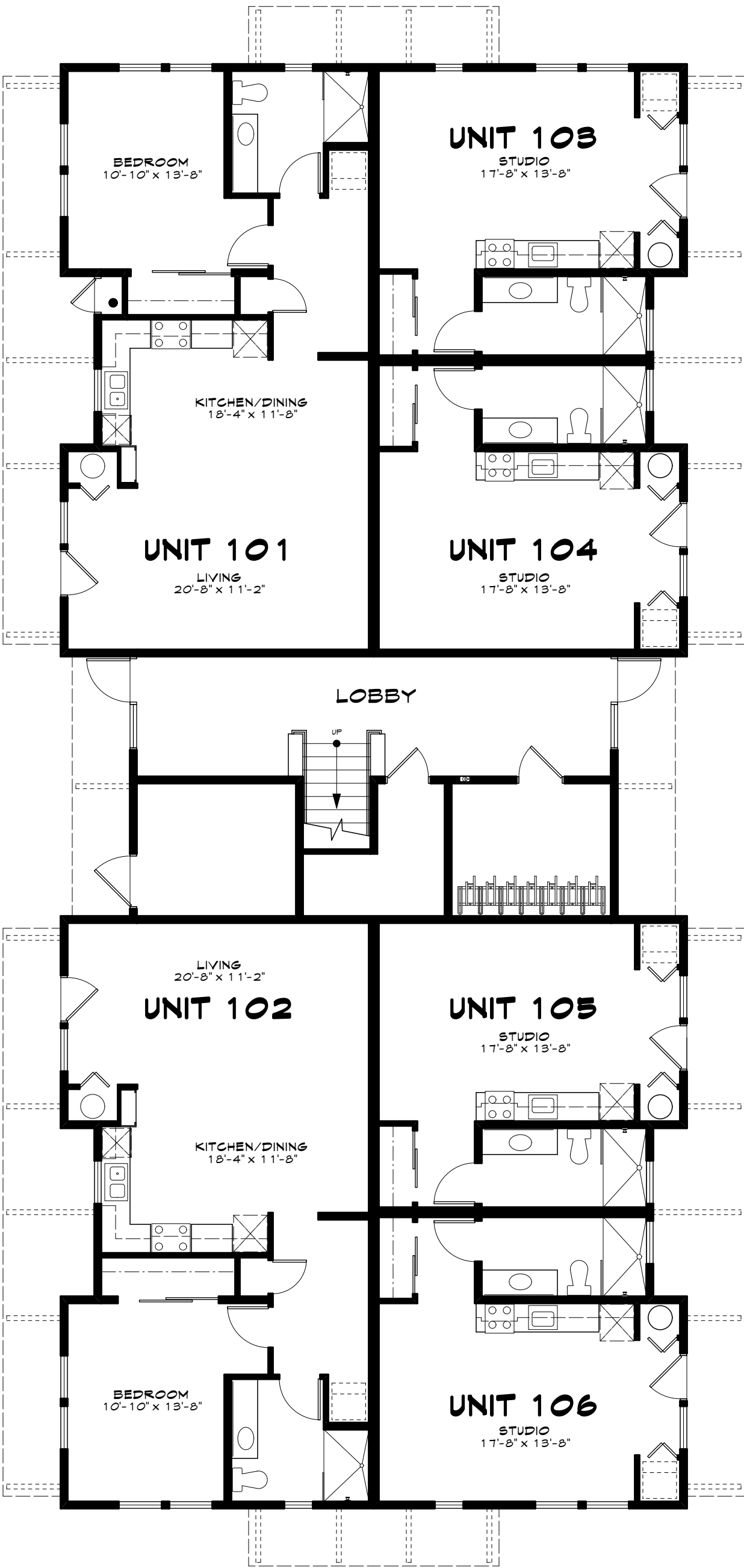
835 EL CAPITAN FIRST FLOOR PLAN
